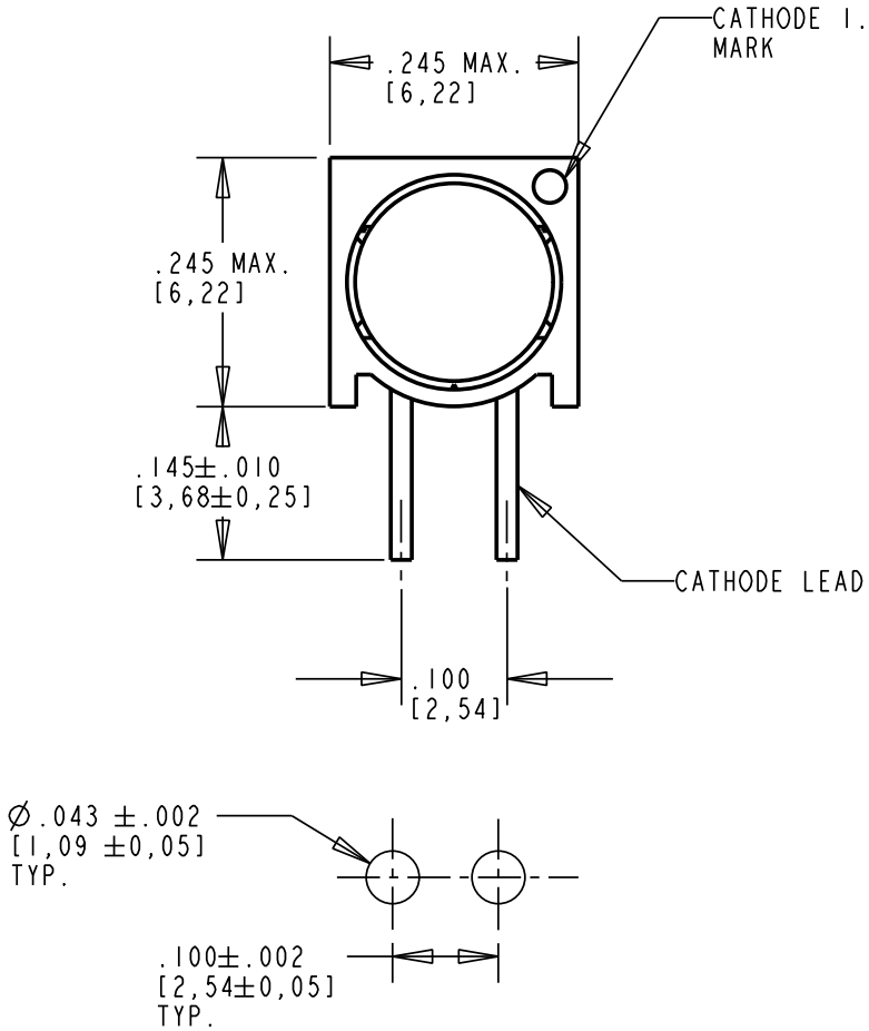
RECOMMENDED PC BOARD HOLE PATTERN
