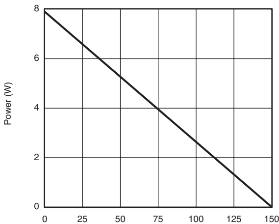
Power, Junction-to-Foot
