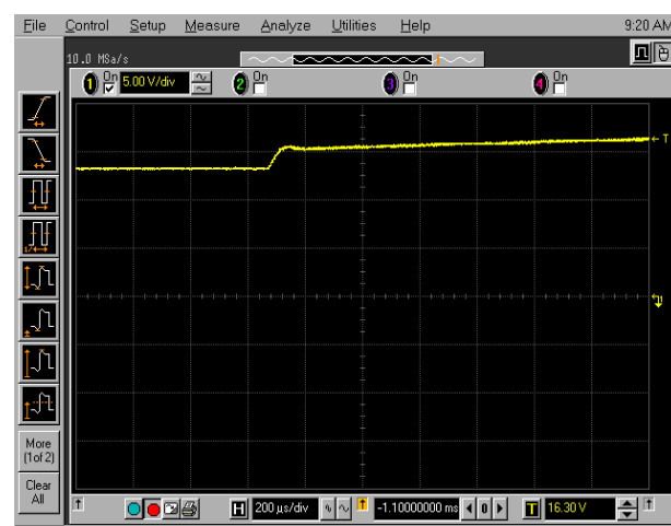
FIGURE 9. VLN TRANSITIONS FROM 13.3V TO 18.3V
