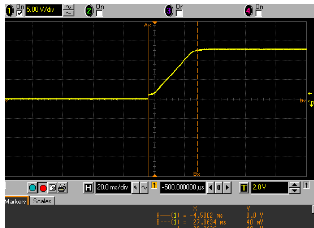
FIGURE 5. VLN RISE TIME WITH T_{CAP} = 0.44\mu\text{F} is 32ms
