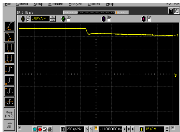
FIGURE 10. V LN B TRANSITIONS FROM 18.3V TO 13.3V
