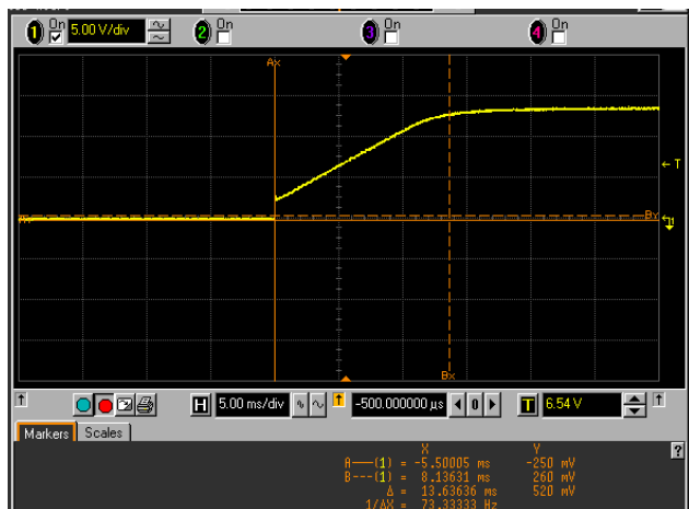
FIGURE 4. VLN RISE TIME WITH T_{CAP} = 0.22\mu\text{F} is 13ms
