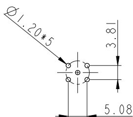
5 Pin Male Connector Male Pin PCB Layout
