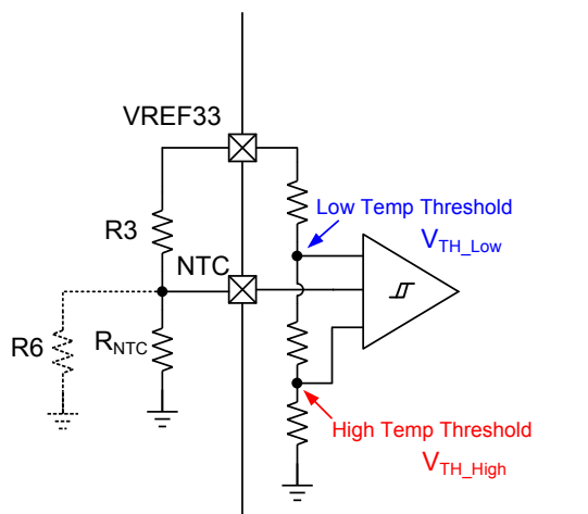
Figure 5— NTC function block
