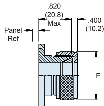
Style 1 Front Mount Type B RFI/EMI (Shown With Style G Gland Nut)
