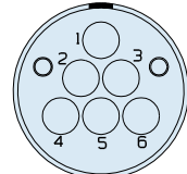
Size 15-06
