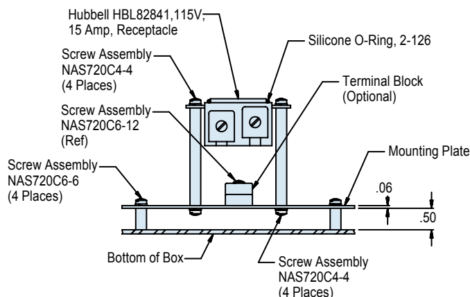
VIEW C-C
