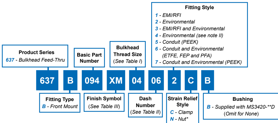
Type B Environmental Style 2
