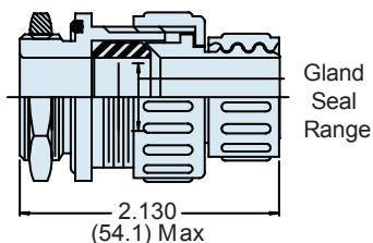
Style E Environmental Conduit Adapter
