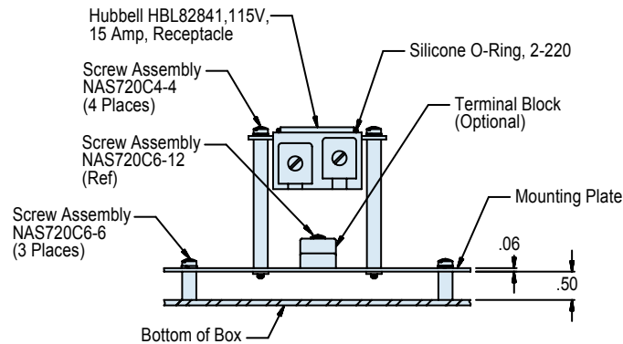
VIEW C-C
