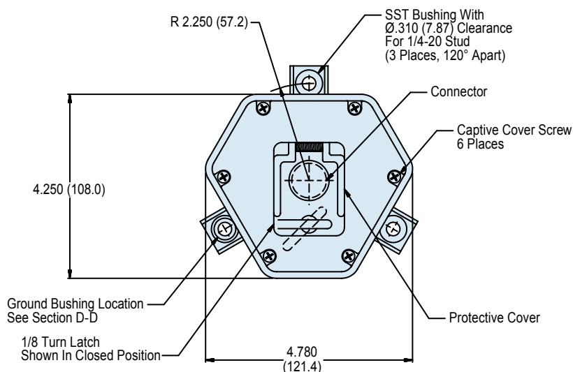
FIGURE 1 TOP VIEW
