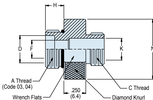
Adapter with Internal Class 2B Thread (Code 03 and 04)
