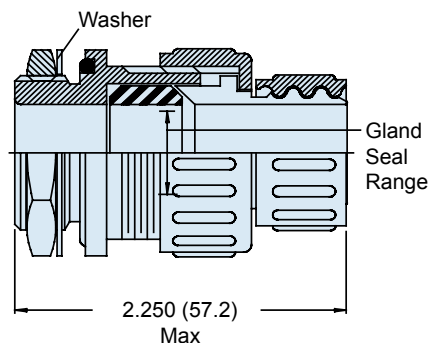
Type B Environmental Conduit Adapter Style 6 or 7
