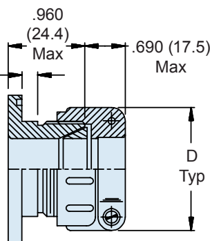
Style 1 Rear Mount Type A RFI/EMI (Shown With Style F Strain Relief)
