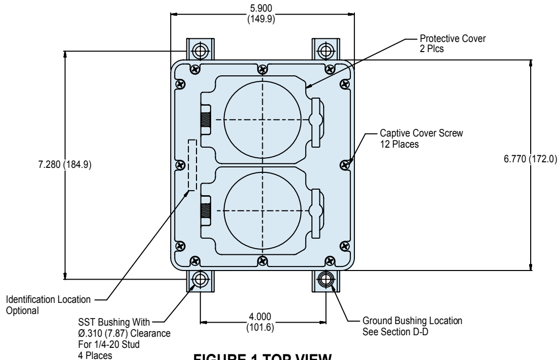
FIGURE 1 TOP VIEW
