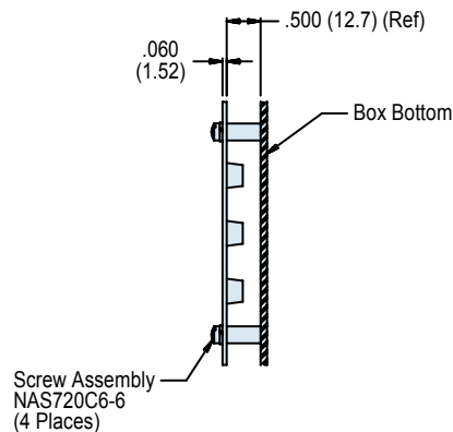
VIEW C-C
