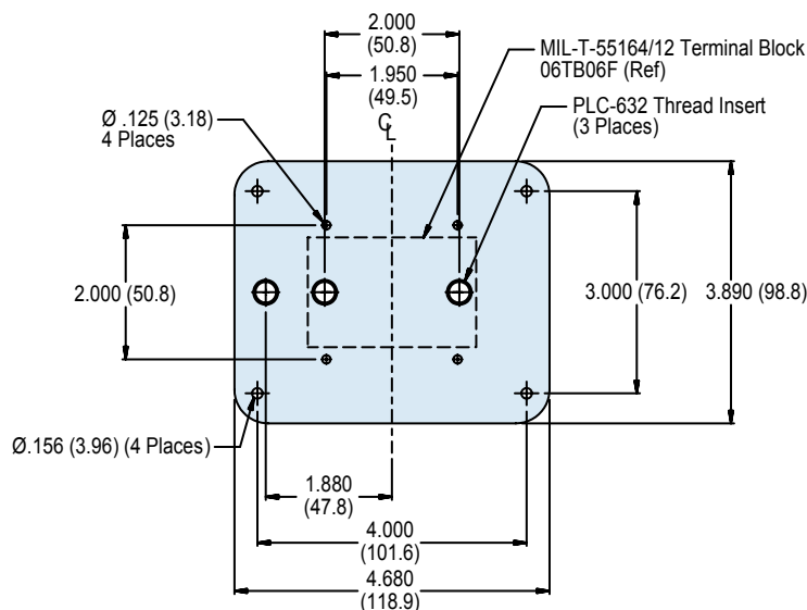
DETAIL B
