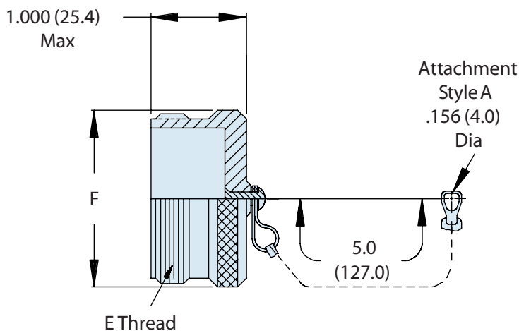
M28840/15 Plug Cover
