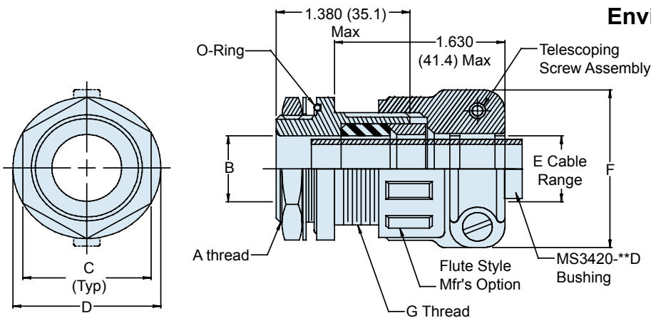
Type B Environmental Style 2
