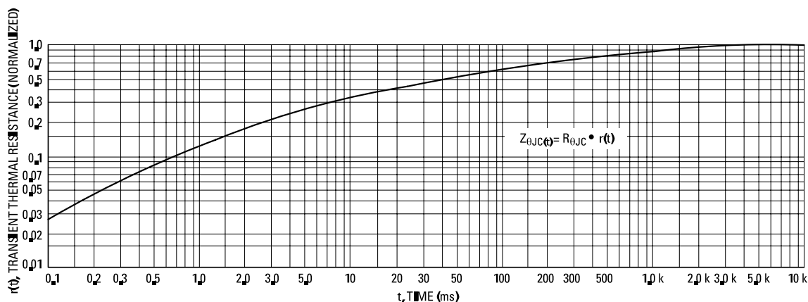
Figure 5. Thermal Response
