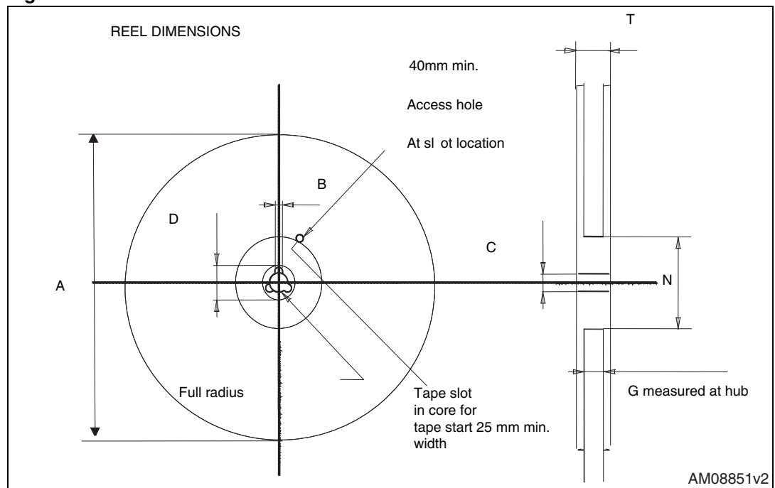
Figure 26. Reel
