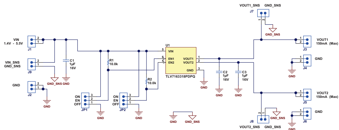
Figure 4. TLV7163318EVM-535 Schematic
