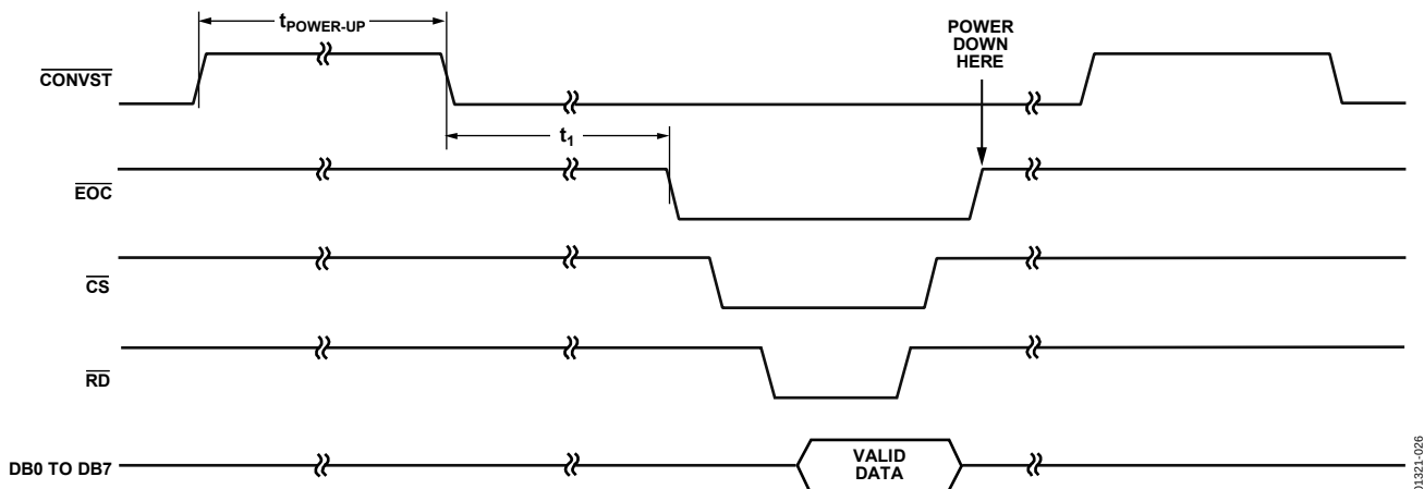
Figure 25. Mode 2 Operation
