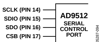
Figure 30. Serial Control Port
