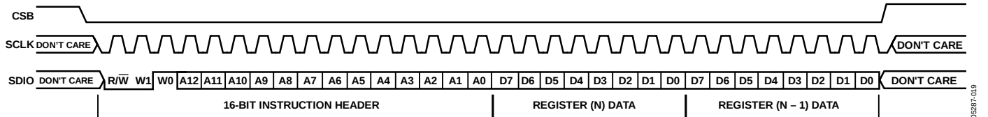
Figure 32. Serial Control Port Write—MSB First, 16-Bit Instruction, 2 Bytes of Data
