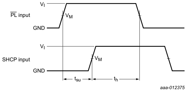
Fig 12. Set-up times for (PL) input to (SHCP) input
