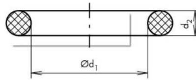
Cross section of recommended O-ring 1
