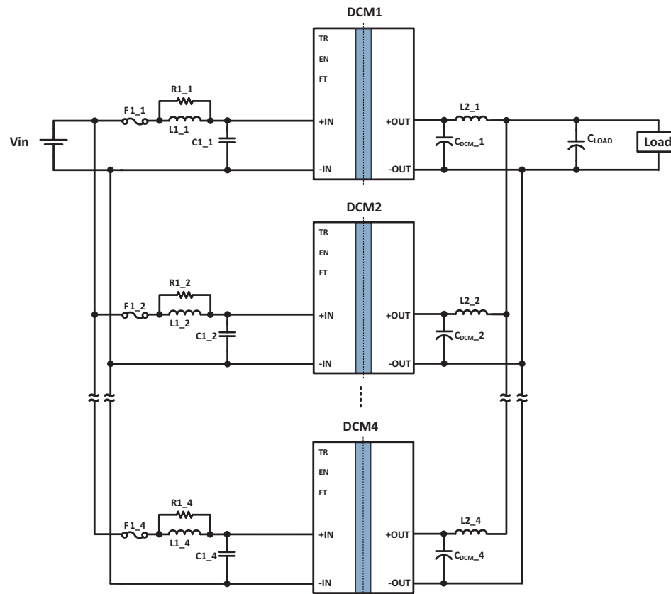
Typical Application 1: MDCM28AP120M320A50 in an array of four units
