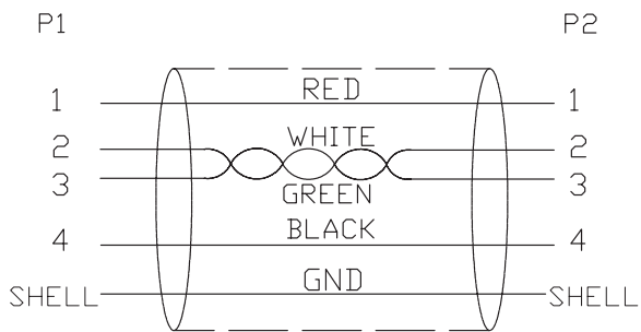
WIRE DIAGRAM
