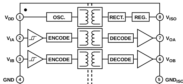
Figure 1. ADuM5240
