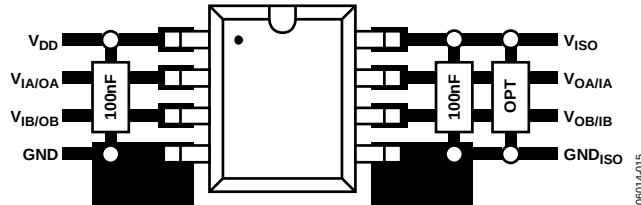
Figure 15. Recommended Printed Circuit Board Layout
