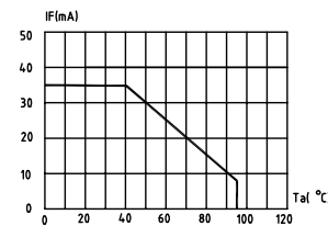
FIG.4b BLUE & GREEN MAXIMUM FORWARD DC CURRENT VS. AMBIENT TEMPERATURE ( T_{jmax}=105^{\circ}\text{C} )
