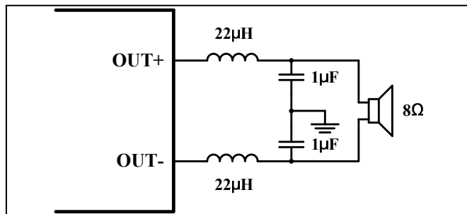
Figure 28 Typical LC Output Filter for 8\Omega Speaker
