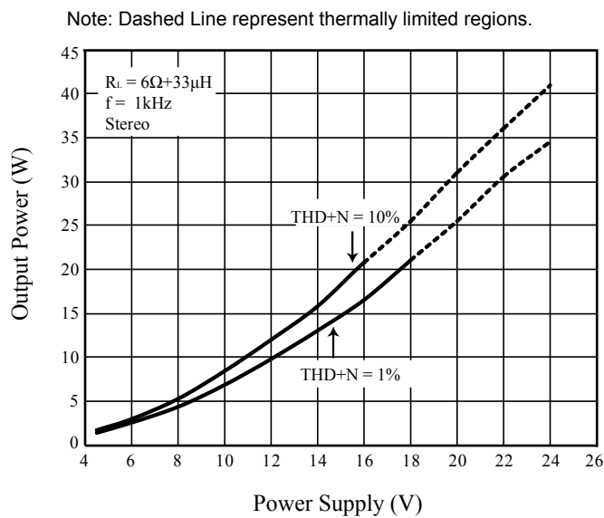
Figure 25 Output Power vs. Power Supply
