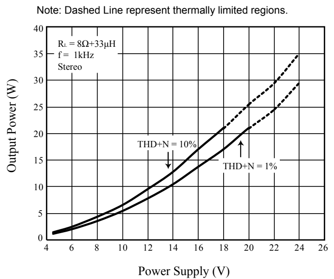
Figure 26 Output Power vs. Power Supply
