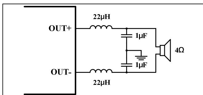
Figure 29 Typical LC Output Filter for 4\Omega Speaker
