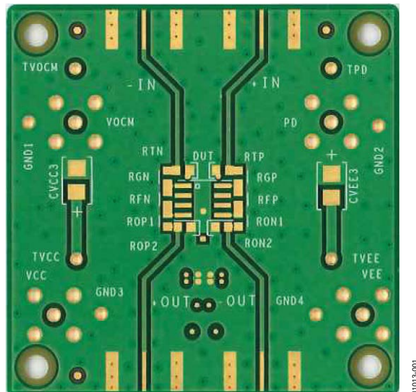
Figure 1. Evaluation Board, Component Side
