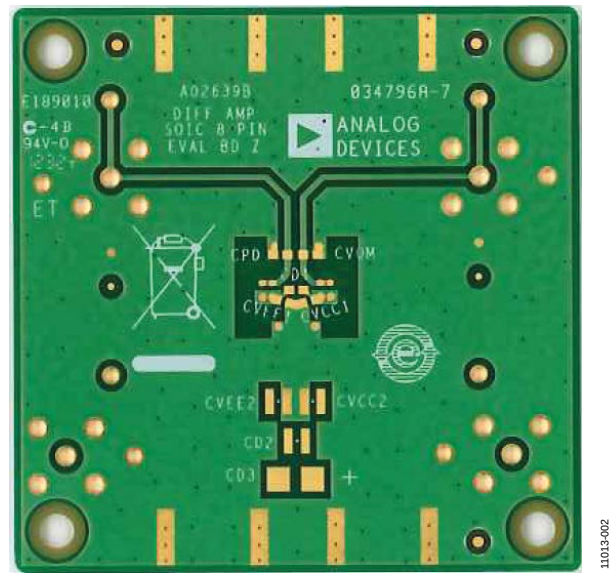
Figure 2. Evaluation Board, Circuit Side
