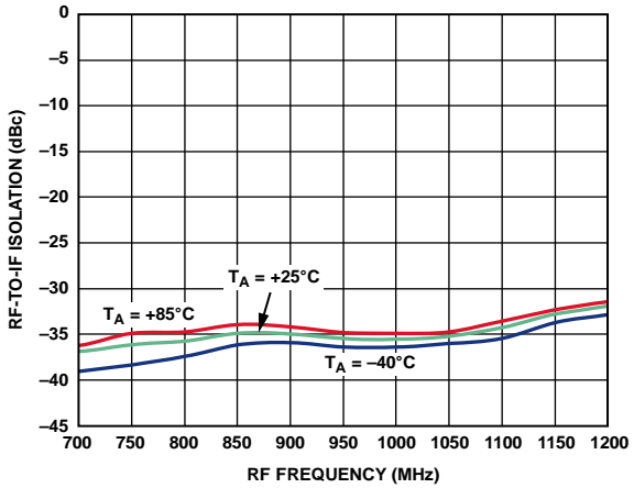
Figure 34. RF-to-IF Isolation vs. RF Frequency
