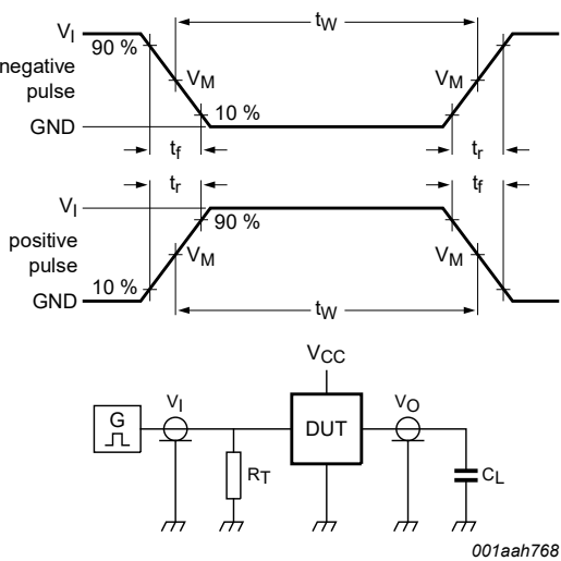
For test data see Table 9 . Definitions for test circuit: R_T = Termination resistance should be equal to output impedance Z_o of the pulse generator. C_L = Load capacitance including jig and probe capacitance.
