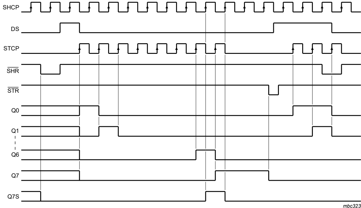
Fig. 8. Timing diagram
