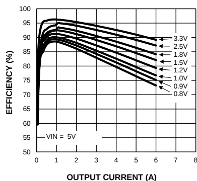
Efficiency ( V_{IN} = 5V ) vs. Output Current
