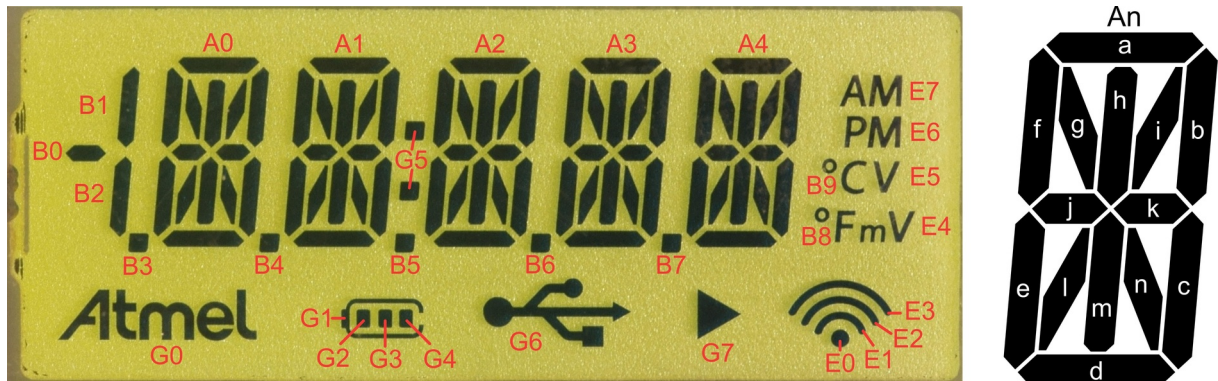
Figure 4-1. YMCC42412AAAFDCL Segments
