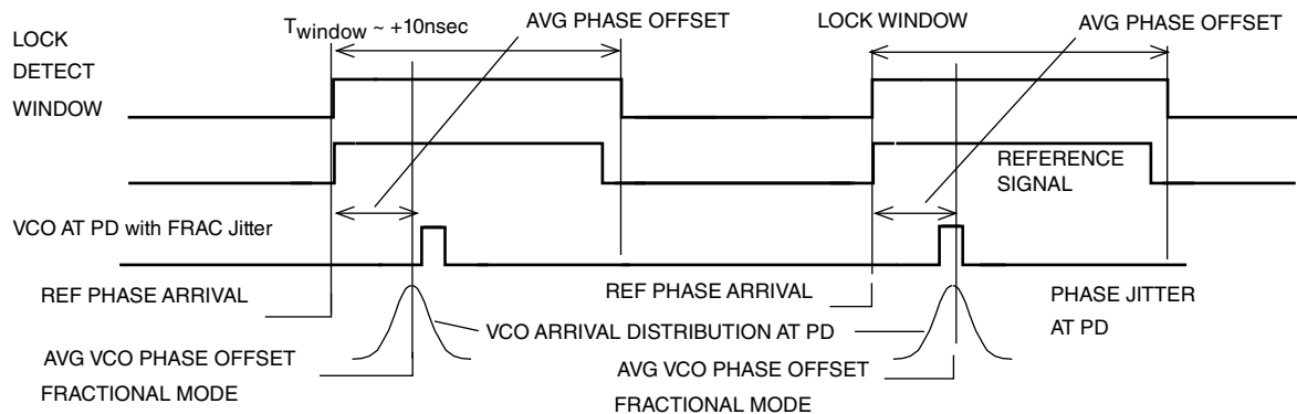
Figure 32. Lock Detect Window - Fractional Mode with Offset
