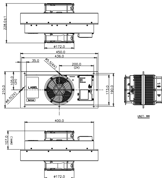
Dimension drawing
