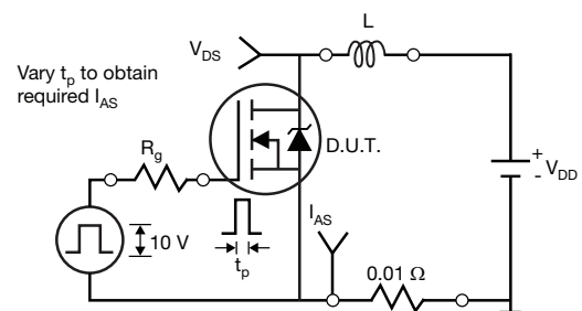
Fig. 16 - Unclamped Inductive Test Circuit
