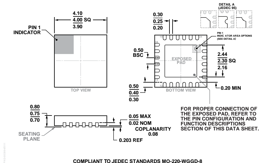
Figure 61. 24-Lead Lead Frame Chip Scale Package [LFCSP] 4 mm × 4 mm Body and 0.75 mm Package Height (CP-24-14)
