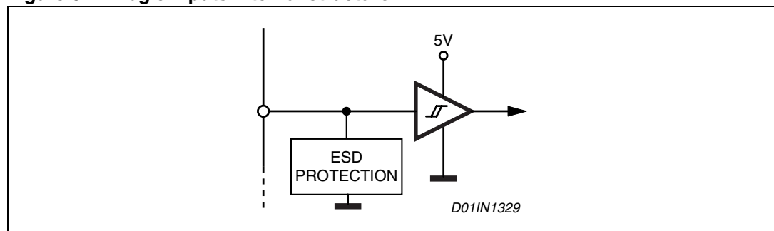
Figure 7. EN_A and EN_B pins open collector driving
