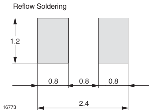
Fig. 11 - Recommended Foot Pads (in mm)
