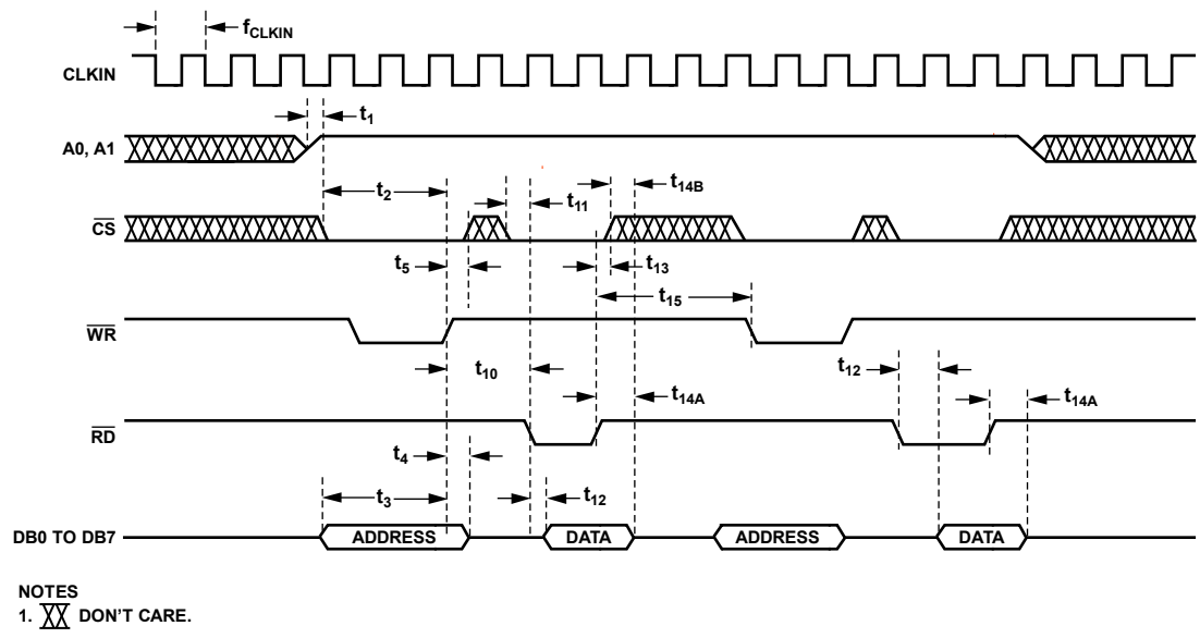
Figure 29. Parallel Port Read Timing—Configuration Mode
