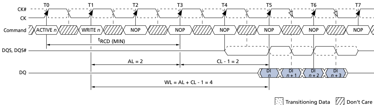
Figure 40: WRITE Latency
