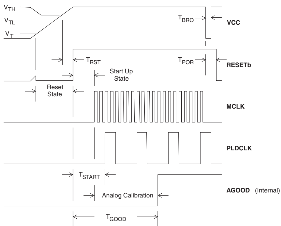
Figure 5-2. LA-ispPAC-POWR1014/A Power-On Reset
