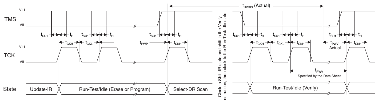
Figure 5-6. Discharge Timing Diagram
