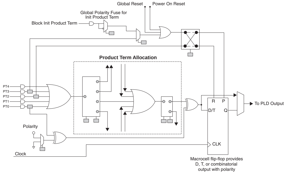
Figure 5-11. LA-ispPAC-POWR1014/A Macrocell Block Diagram
