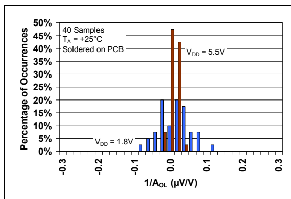
FIGURE 2-11: DC Open-Loop Gain.
