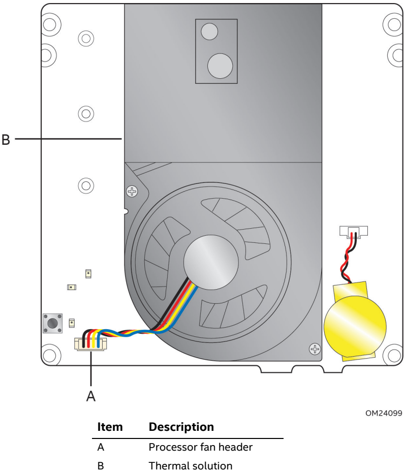
Figure 7. Thermal Solution and Fan Header
