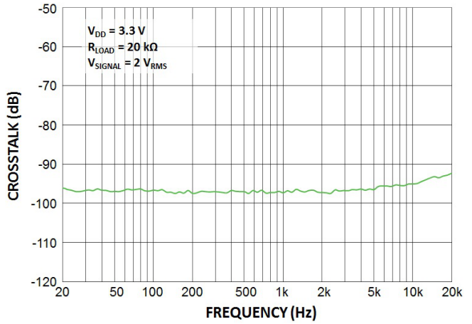
Figure 15. Channel-to-Channel Crosstalk
