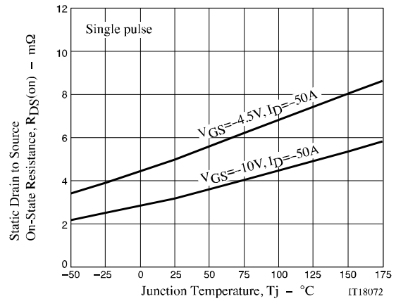
Figure 4. R_{DS(on)} - T_j
