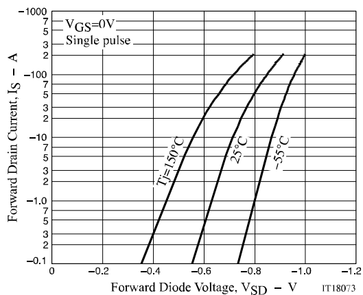
Figure 5. I_S - V_{SD}
