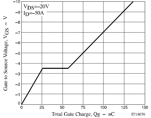
Figure 8. V_{GS} - Q_g
