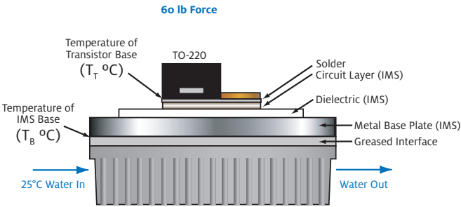
Water-cooled Heatsink
