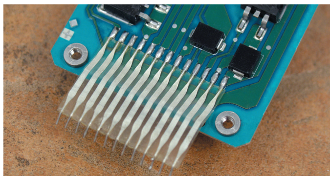
Flex attachment on THERMAL CLAD.
