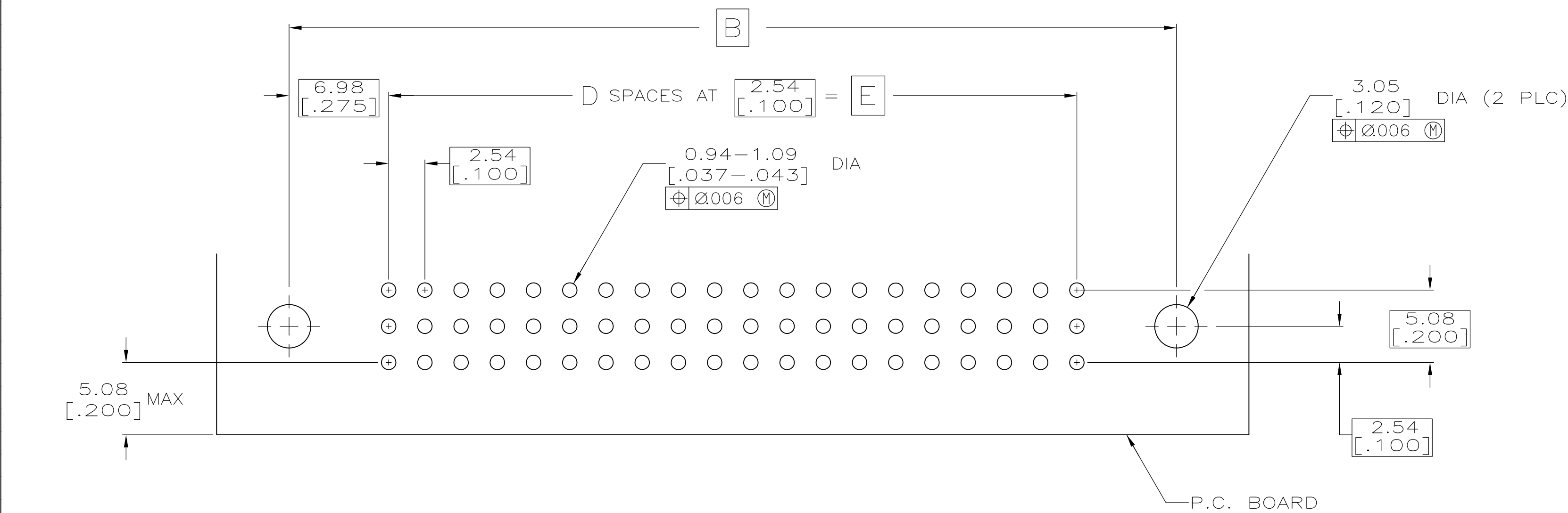
P.C. BOARD
