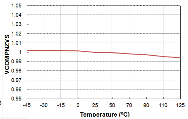
Figure 53. VCOMPZVS vs. Temperature
