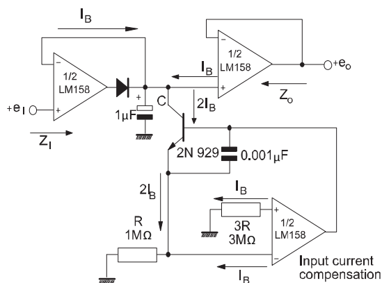
Figure 26: Low drift peak detector
