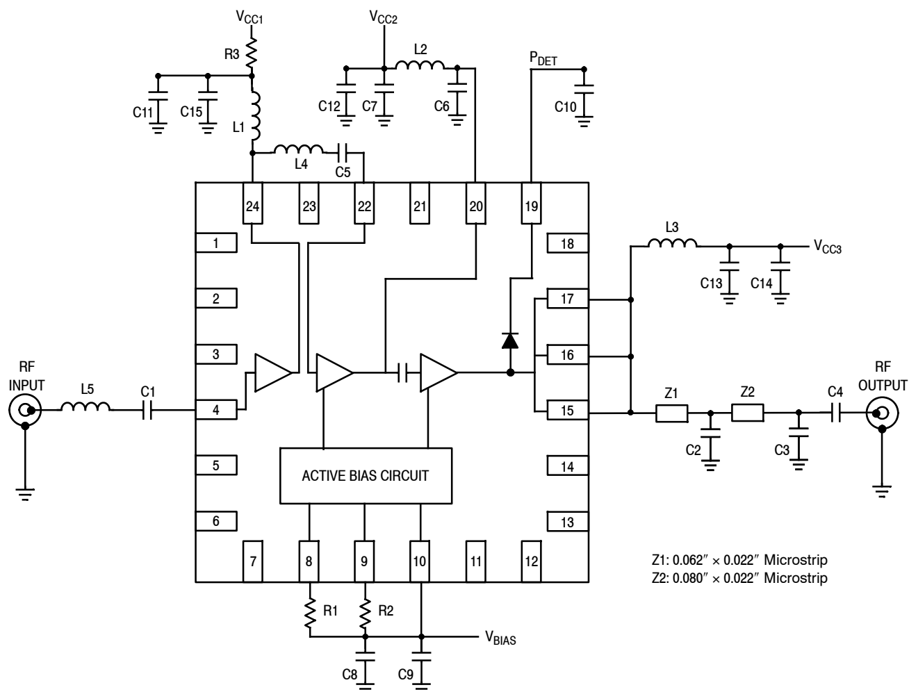
Figure 3. MMZ3833BT1 Test Circuit Schematic
