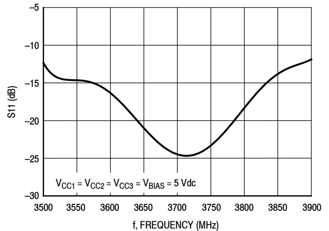
Figure 28. S11 versus Frequency
