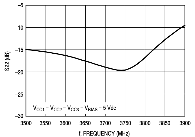
Figure 32. S22 versus Frequency
