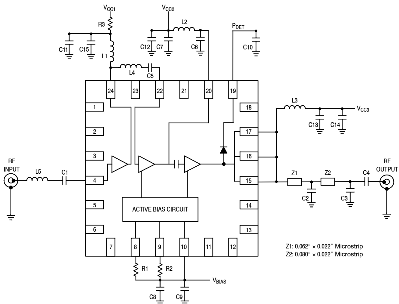
Figure 5. MMZ3833BT1 Test Circuit Schematic
