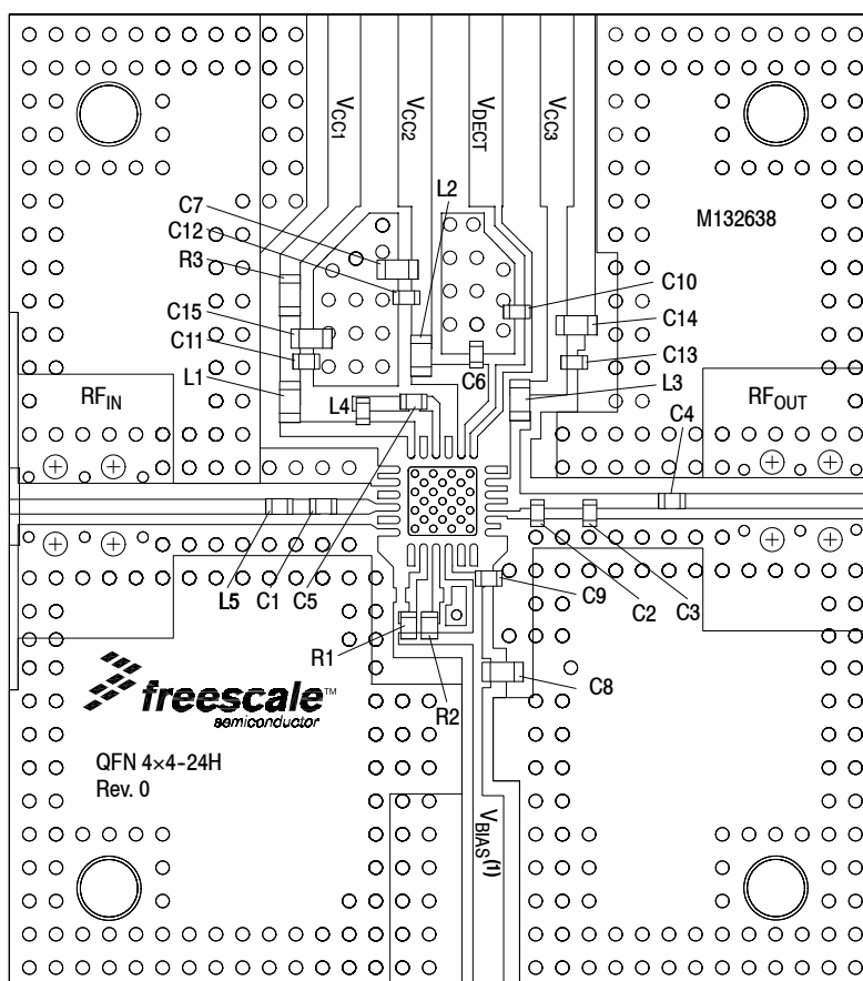
Figure 6. MMZ38333BT1 Test Circuit Component Layout
