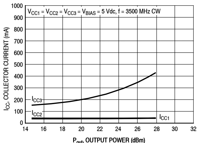
Figure 14. Stage Collector Current versus Output Power
