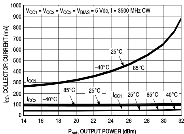
Figure 13. Stage Collector Current versus Output Power versus Temperature
