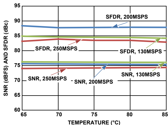
FIGURE 32. TYPICAL SNR AND SFDR PERFORMANCE vs TEMPERATURE, DEVICE CALIBRATED AT +85^{\circ}\text{C} , f_{\text{IN}} = 105\text{MHz}
