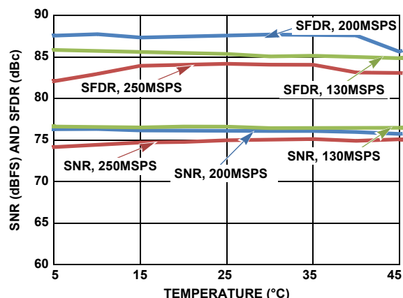
FIGURE 31. TYPICAL SNR AND SFDR PERFORMANCE vs TEMPERATURE, DEVICE CALIBRATED AT +25^{\circ}\text{C} , f_{\text{IN}} = 105\text{MHz}
