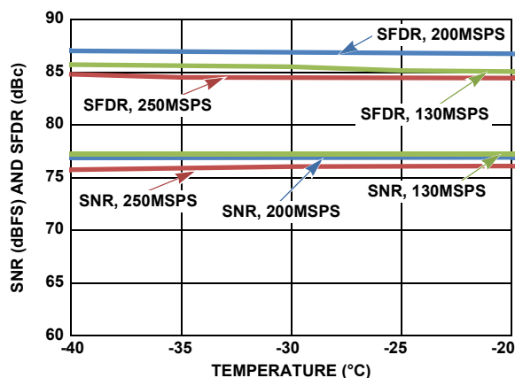
FIGURE 30. TYPICAL SNR AND SFDR PERFORMANCE vs TEMPERATURE, DEVICE CALIBRATED AT -40^{\circ}\text{C} , f_{\text{IN}} = 105\text{MHz}
