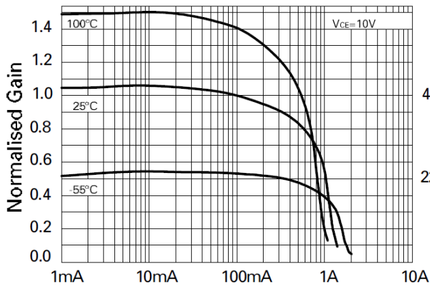
Collector Current
