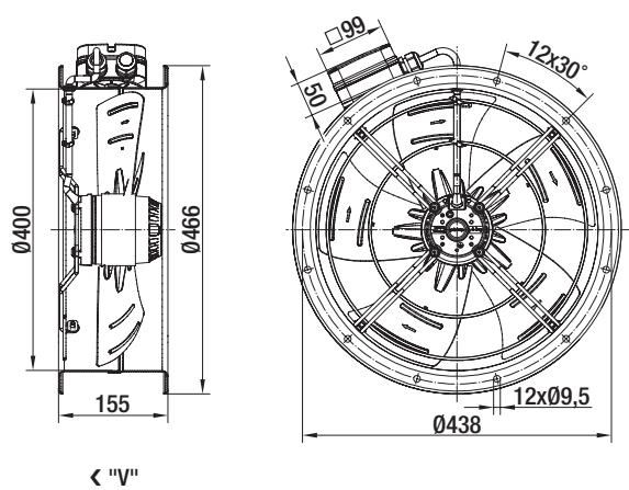
In-line duct fan
